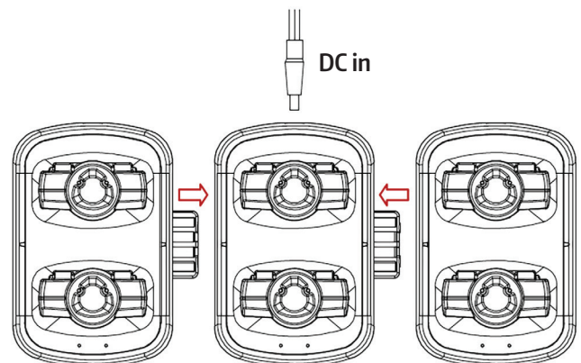
Sharing power with another 2 x HC2 chargers
