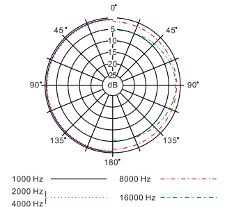
Polar Pattern
