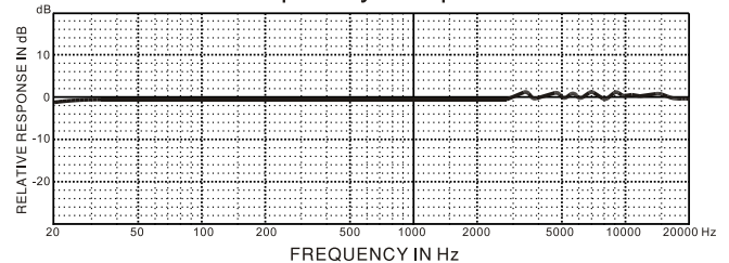
Frequency Response
